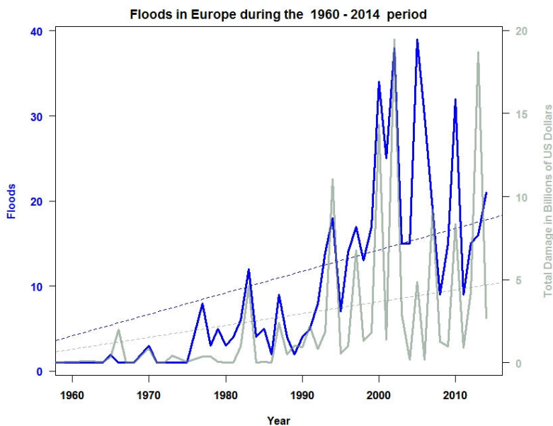
Figure 1: Floods and flood-related damages in Europe for the 1960-2014 period. The frequency of floods is shown in blue, while the total damages related to floods are shown in green colour. The two dashed lines are a linear fit to the data and represent a trend of an increasing flood frequency and total damage costs. The data are taken from emdat.be.
