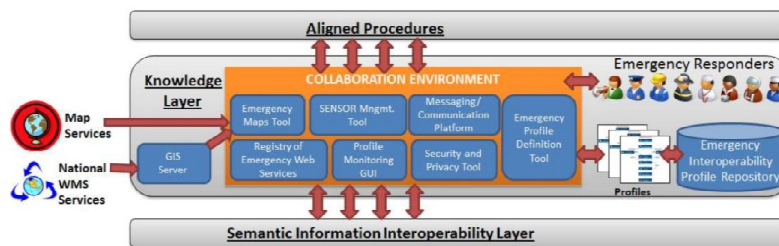
Figure 4: The Knowledge Layer, where all incoming information is put into final processing for presentation on maps. The data are enriched and presented in such a way that it eases decision making.
